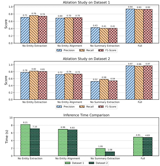
Fig. 8: Ablation Study of AetherLog’s Components
