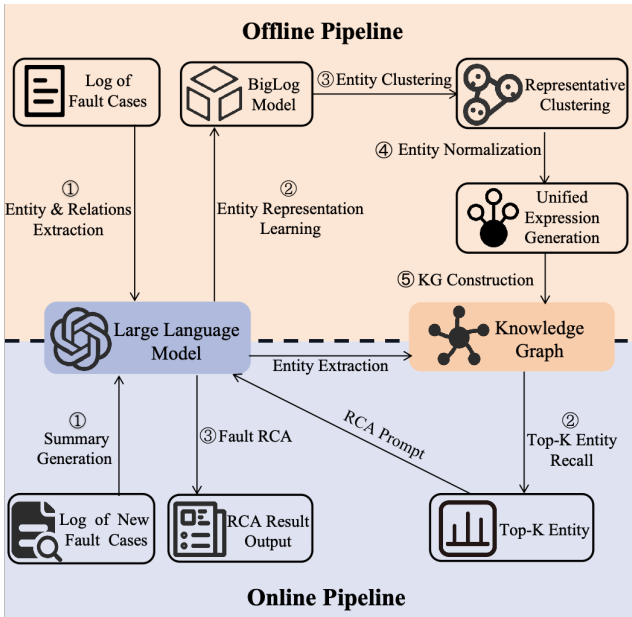
Fig. 3: The framework of AetherLog
