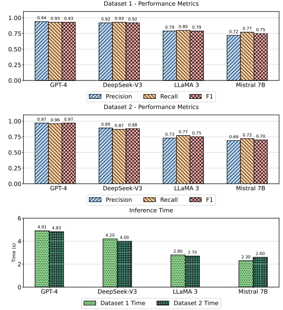
Fig. 7: Performance comparison of different LLMs.
