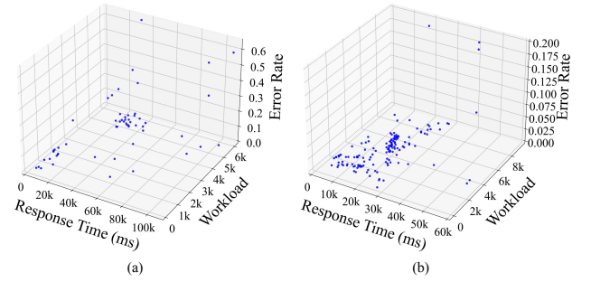
Figure 3: Distributions of SUT performance at the breaking point across three dimensions: workload, response time, and error rate. (a) Data from dataset D1; (b) Data from dataset D2. Each point represents a unique test case.
