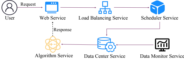
Figure 10: The workflow of PerfScout in Huawei Cloud industrial environment.
