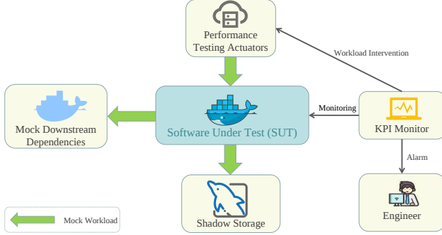
Figure 4: System architecture of software performance testing. Actuators generate mock workloads while the monitor collects real-time KPIs to detect anomalies.
