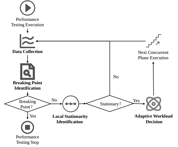
Figure 5: The overall framework of PerfScout , illustrating its four core modules: data collection, breaking point identification, local stationarity identification, and adaptive workload decision.
