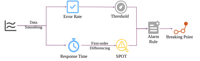
Figure 6: Workflow of breaking point identification. After smoothing the incoming KPI data, PerfScout checks whether the error rate exceeds a fixed threshold and applies first-order differencing and SPOT to detect abrupt changes in response time. An alarm rule then integrates both signals to confirm the breaking point.
