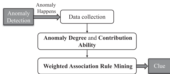
Fig. 3. The overview of RobustSpot.
