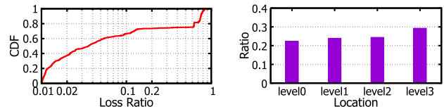
Fig. 1. Loss rate and location distribution of lossy links (loss rate > 1%) in a production DCN. Level0-3 denote server↔ToR, ToR↔Agg, Agg↔Spine, and Spine↔Core, respectively.
