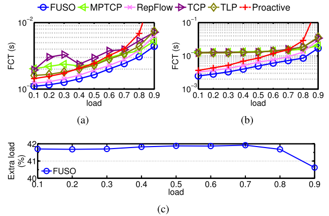
Fig. 7. Failure & congestion loss: Average and 99 th FCT (log scale) of latency-sensitive flows, and the average extra load of all FUSO flows. Each flow's extra load is calculated by the extra bytes incurred by FUSO divided by the total bytes transmitted . (a) Avg FCT. (b) 99 th FCT. (c) Extra load in FUSO.
