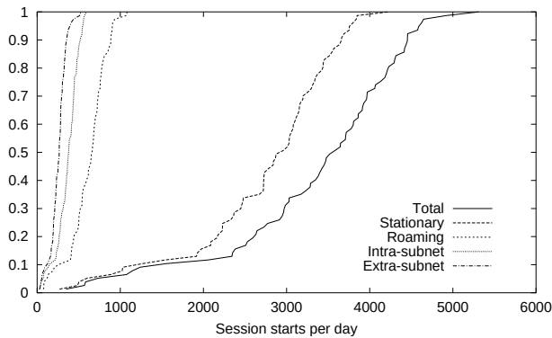
Figure 14: [syslog] Number of session starts per day, distribution over days. Median is 3582 sessions, or 664 roaming sessions.
