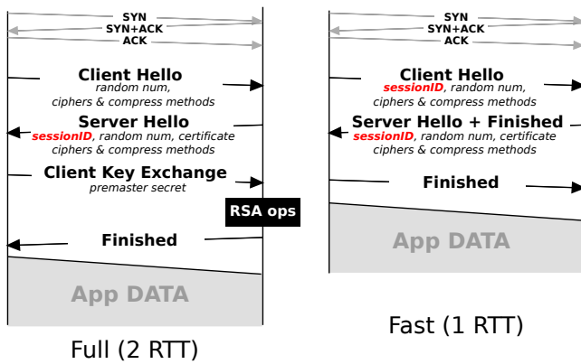
Figure 2: SSL/TLS negotiation.
