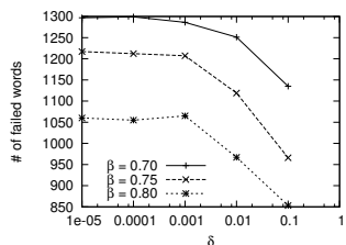
Fig. 5. Comparison of the number of false positive words.
