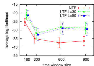
Fig. 8. Comparison of the average of test log likelihood with different L and time-window sizes and K = 60 . Error bars represent the 95% confidence interval of a mean.
