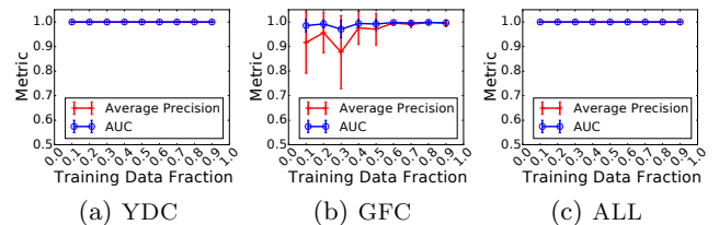
Figure 8: AP and AUC with varying training % p .
