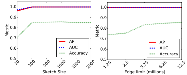
Figure 13: STREAMSPOT performance on ALL with (left) sketch size L and (right) memory limit N .
