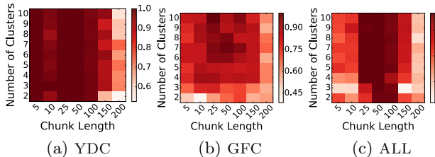
Figure 6: Average precision for different chunk-length C and number of clusters K . ( p = 75\% )
