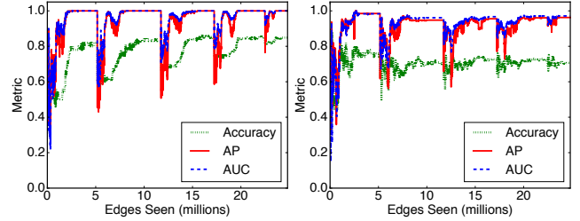
Figure 11: Performance of STREAMSPOT on ALL for different values of the sketch size.
