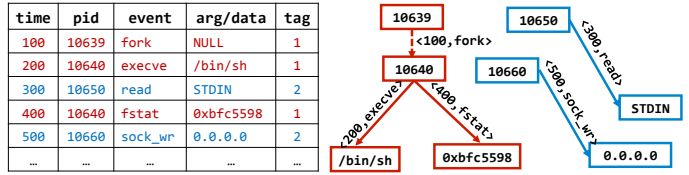
Figure 1: Example stream of system logs, and two resulting information flow graphs (red vs. blue). Both nodes and edges are typed. Edges arriving to different flows may interleave.
