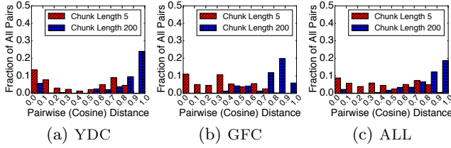
Figure 4: Distribution of pairwise cosine distances for different values of chunk lengths.
