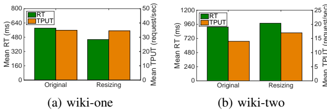
Fig. 13: Performance comparison for wiki-one and wiki-two: original and resized with ATM.
