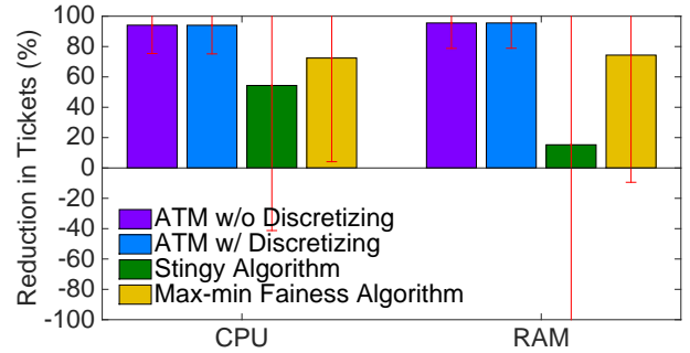
Fig. 8: Ticket reduction for CPU and RAM: comparing ATM, max-min fairness, and stingy algorithms.
