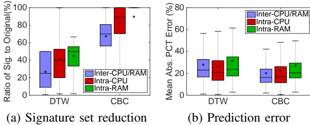
Fig. 7: Comparison of inter- and intra-resource models.
