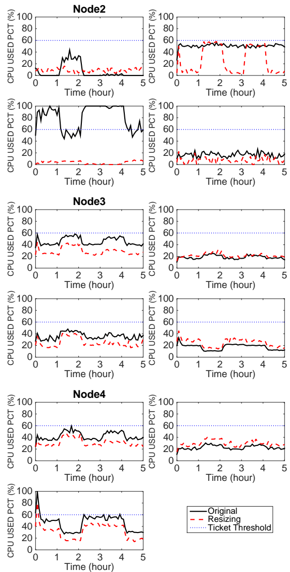
Fig. 12: Overtime plots of CPU utilization for VMs located on Node 2, 3 and 4, with and without resizing.
