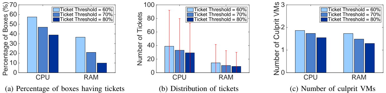
Fig. 2: Characterization of usage tickets for CPU and RAM of VMs per box.
