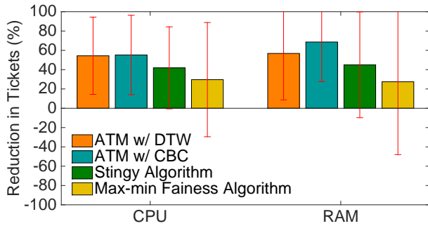
Fig. 10: Comparing ticket reduction: ATM, max-min fairness, and stingy resizing algorithms.
