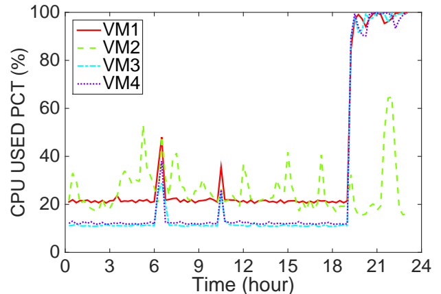
Fig. 1: An illustration of spatial dependency across usage time series for 4 VMs co-located on a box.
