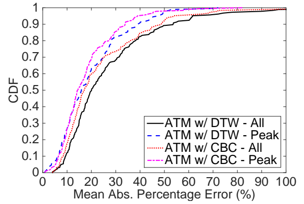
Fig. 9: CDF of prediction accuracy of ATM on 400 production servers: ATM_{CBC} , ACM_{DTW} .
