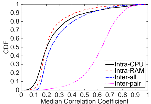
Fig. 3: Cumulative distribution of correlation of intra-CPU, intra-RAM, inter-CPU/RAM.
