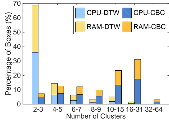
Fig. 5: Comparison of clustering results using DTW and CBC.
