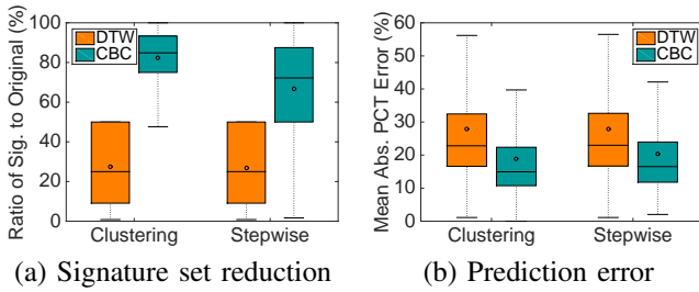
Fig. 6: Comparison of the two steps: effectiveness of clustering and stepwise regression.
