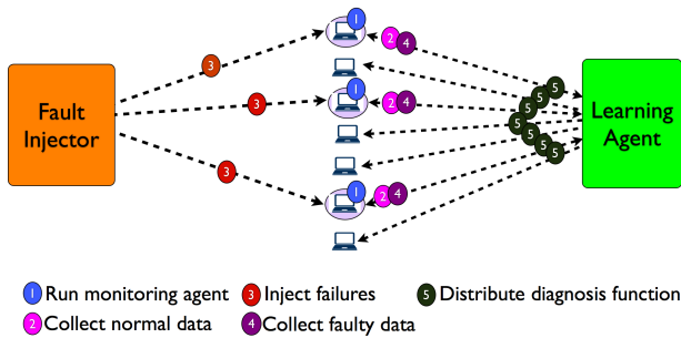
Figure 1: Overview of NetPoirot
