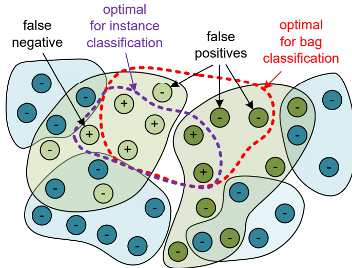
Figure 2: Illustration of two decisions boundaries on a fictive problem. While only the purple boundary correctly classifies all instances, both them achieve perfect bag classification. This is because, in that case, false positive and false negative instances do not impact on bag labels.
