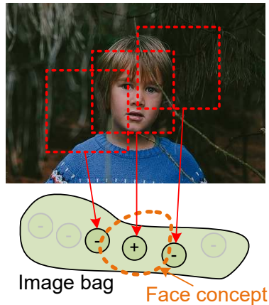
Figure 3: Illustration of intra-bag similarity between instances: The patches are overlapping, and thus, share similarities with each other.
