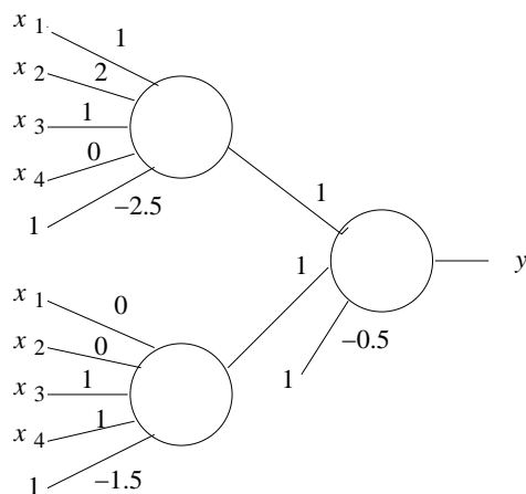
Figure 13.2: Making the threshold 0 for all nodes
