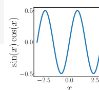
Figure 3.8 f(x) = \sin(x)\cos(x) .
