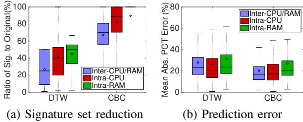
Fig. 7: Comparison of inter- and intra-resource models.
