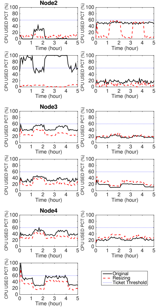
Fig. 12: Overtime plots of CPU utilization for VMs located on Node 2, 3 and 4, with and without resizing.
