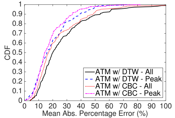
Fig. 9: CDF of prediction accuracy of ATM on 400 production servers: ATM_{CBC} , ATM_{DTW} .
