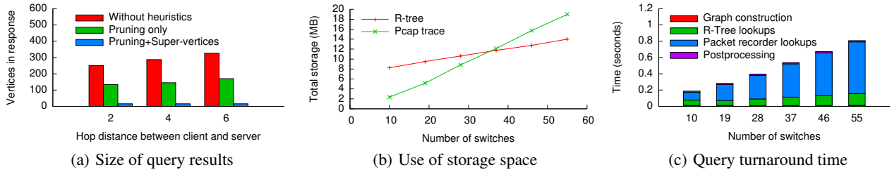
Figure 13: Scalability results
