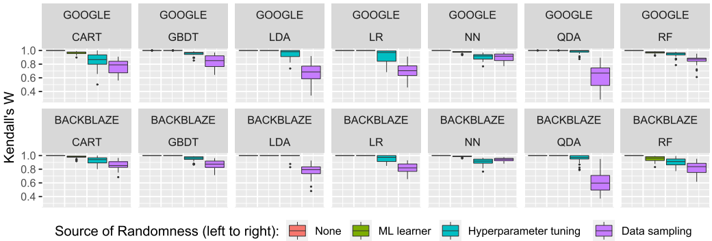
Fig. 6. The interpretation consistency (measured by Kendall's W) of models when different sources of randomness are not controlled. Each subplot has four boxplots, from left to right, representing the control group (all sources of randomness controlled), randomness from ML learner, hyperparameter tuning, and data sampling. See Table 4 for detailed setup.
